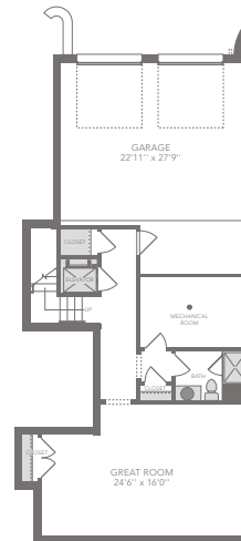
BASEMENT & GARAGE
